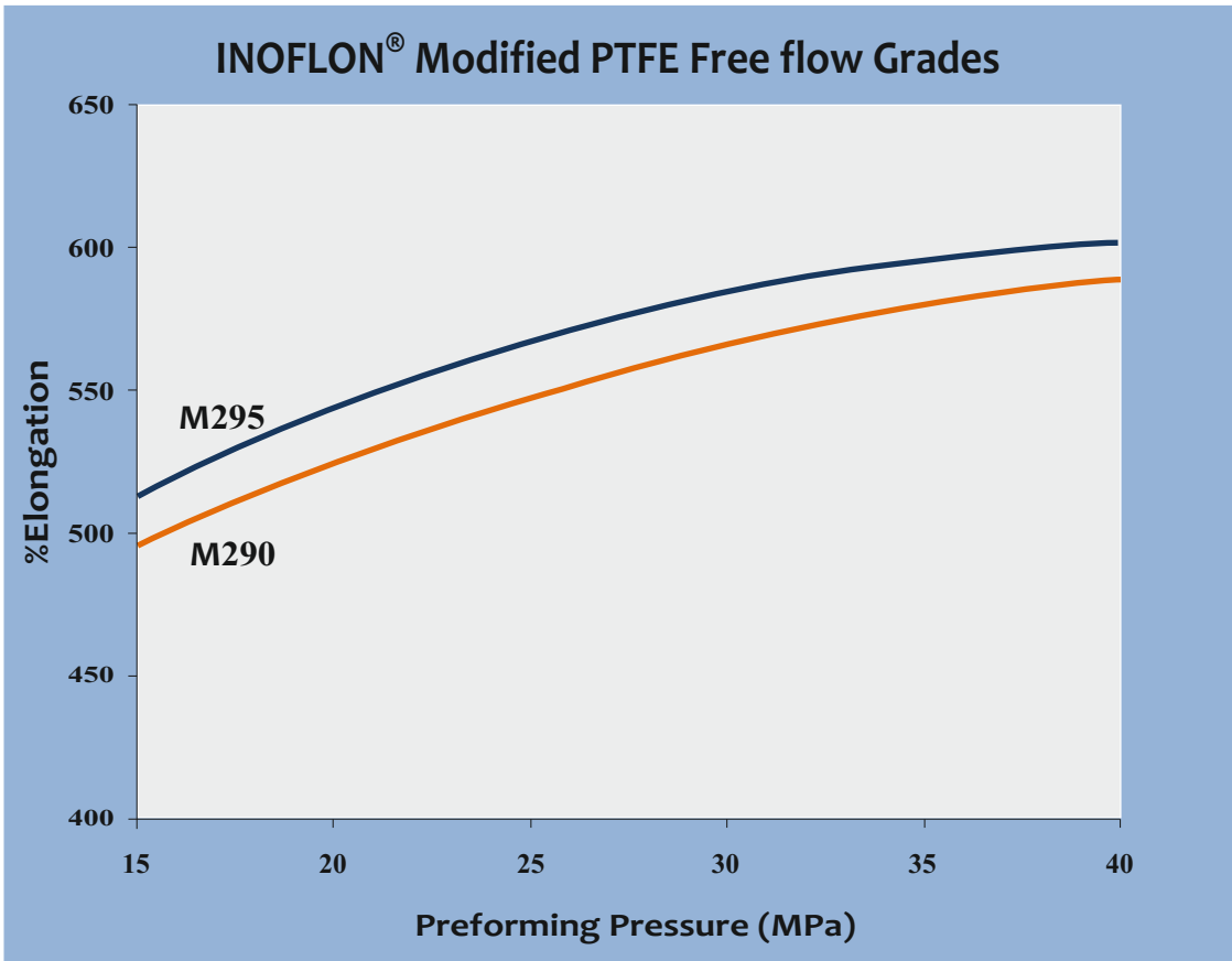
Figure 4 - Effect of preforming pressure on elongation of INOFLON® Free flow granular modified PTFE grades
