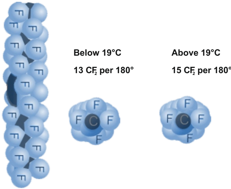
Figure 2- Transition of modified PTFE Molecule
