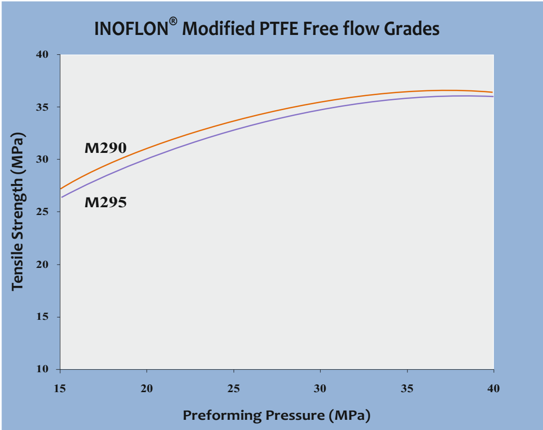
Figure 3 - Effect of preforming pressure on tensile strength of INOFLON® Free flow granular modified PTFE grades
