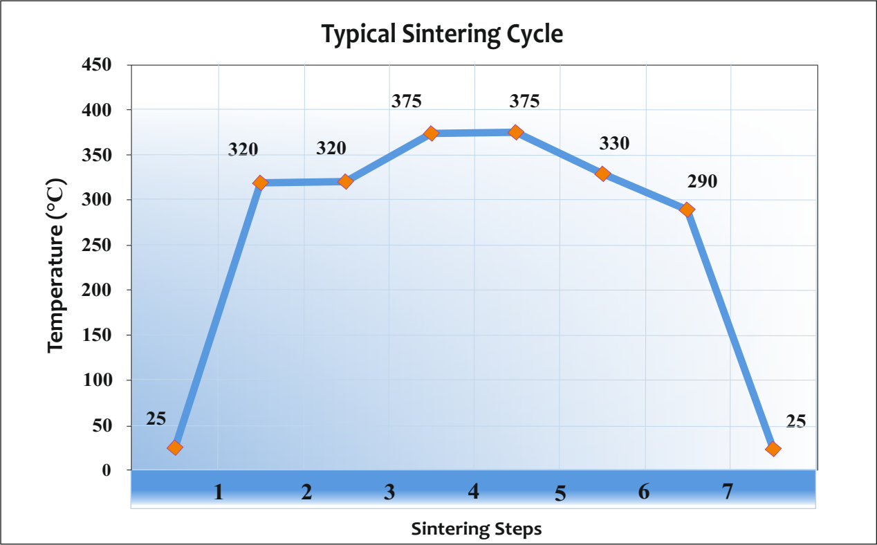
Figure 7- Typical sintering cycle for INOFLON® Free flow granular modified PTFE, Solid billets (Ref. - Table 3)
